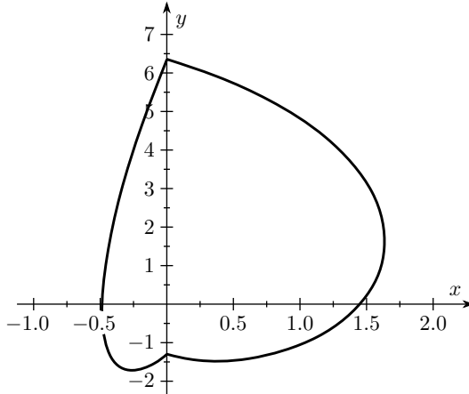
Figure 1. The crossing non-algebraic limit cycle of the discontinuous piecewise linear differential systems (10).
